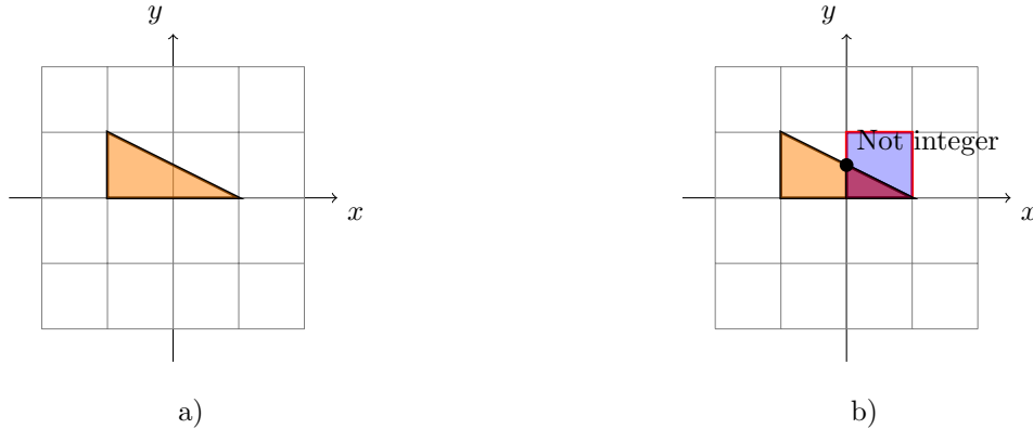
Figure 1.11: a) An integer polytope in \mathbb{R}^2 ; b) Shows that such polytope is not box-integral.
