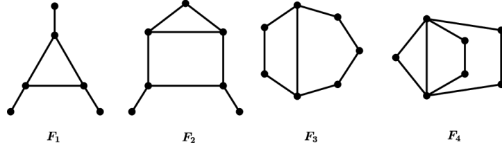
Figure 3.9: Forbidden subgraphs for the box-TDIness of the matching polytope. All the credits of this image are due to the authors of [29].
