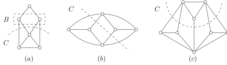
Figure 1.6: (a) A barrier cut C with respect to the barrier B ; (b) A 2-separation cut; (c) A tight cut which is not an ELP-cut. All the credits of this image are due to the authors of [27].
