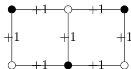
Figure 1.12: Counterexample to the converse of Theorem 1.39.
