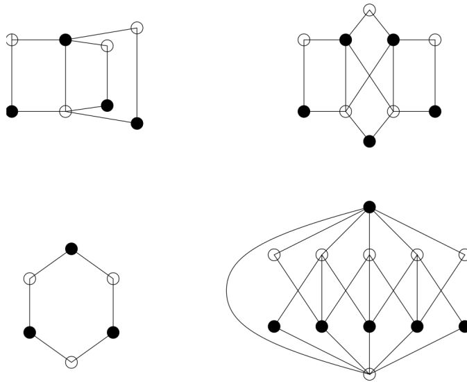
Figure 2.3: Graphs whose bipartite representation is minimally nontotally unimodular. This image has been taken from [19, Page 58] and all the credits are due to the author.
