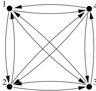
Figure 1: Diclique K_4
