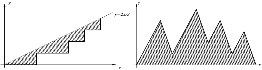
Fig. 3: A walk with below the line y = 2x/3 is mapped to an excursion: Each jump (1, 0) (resp. (0, 1) ) is mapped to a jump (1, 2) (resp. (1, -3) ).
