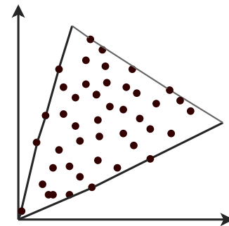
FIGURE 4.2: An example of \bar{V} polytope including vector-valued functions for VMDPs with two objectives.
