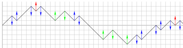
Fig. 3. Flips can increase the number of mismatches (red arrows), let it unchanged (blue arrows) or decrease it (green arrows). The two last are respectively called reversible and irreversible flips: they are the only ones performed during the cooling process.
