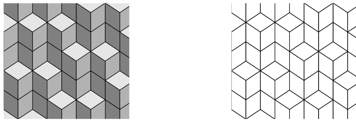
Figure 3. From a stepped plane to a tiling of the plane \Delta by three kind of lozenges.
