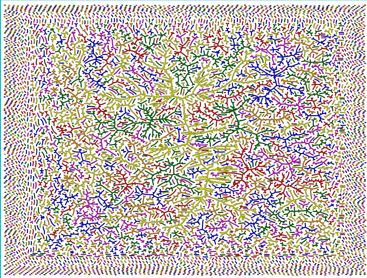
A critical graph of 40000 nodes; the giant component is a huge tree [credit N.Broutin]
