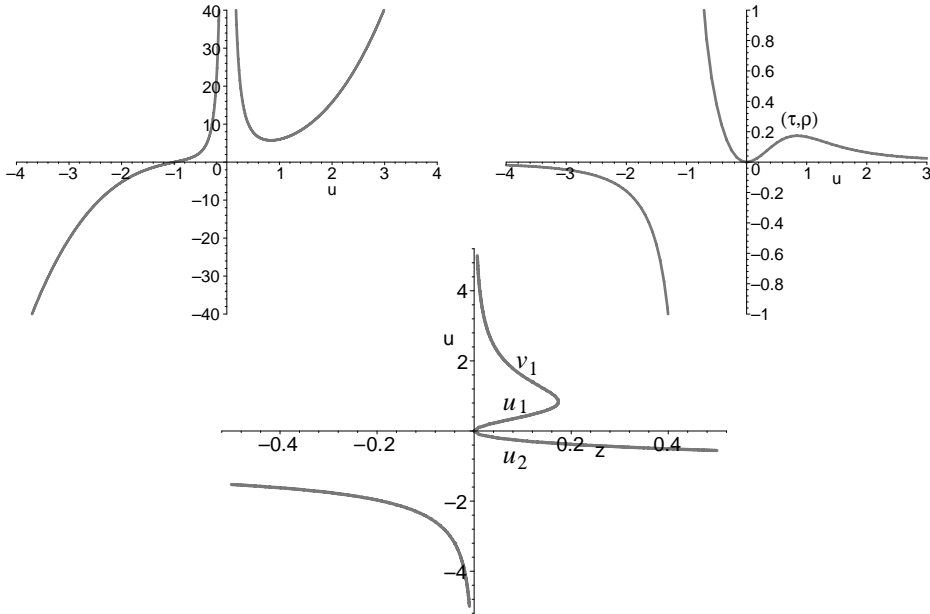
Fig. 3. Graphs associated to the set of jumps \mathcal{S} = \{-2, -1, 0, 1, 2, 3\} , with characteristic polynomial P(u) = u^{-2} + u^{-1} + 1 + u + u^2 + u^3 . Top: the graphs of P(u) and 1/P(u) for real u . Bottom: the three real branches of the characteristic curve, one large of order z^{-1/3} , and two small of order \pm z^{1/2} (two complex branches of order e^{\pm 2i\pi/3} z^{-1/3} are not shown).
