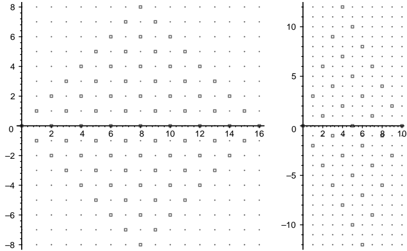
Fig. 2. Fragments of the sublattices accessible from the origin by the Dyck walk ( \mathcal{S} = \{-1, +1\} ) and Duchon’s clubs ( \mathcal{S} = \{-2, +3\} ). The periods are 2 and 5, respectively.
