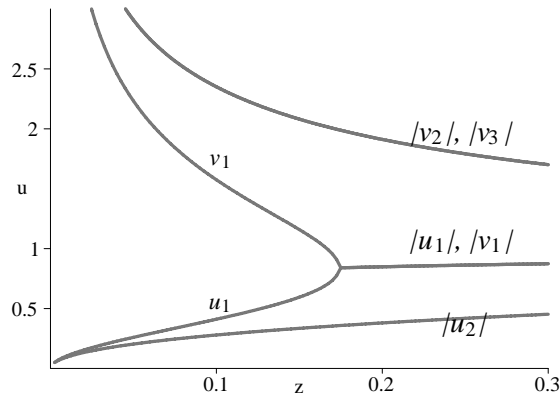
Fig. 4. A rendering of the modulus of the five branches of the characteristic curve in the example of Fig. 3 illustrates the domination properties of the principal small and large branches.
